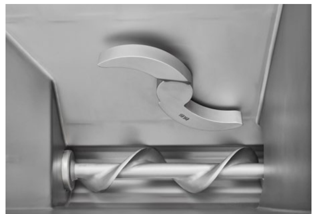
Stirring/feeding device. To secure continuous infeed of difficult/sticky meat raw material of the grinder worm/auger.
