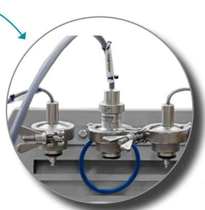
Close-up picture of inlet and outlet temperature sensors as well as pressure transducers.
