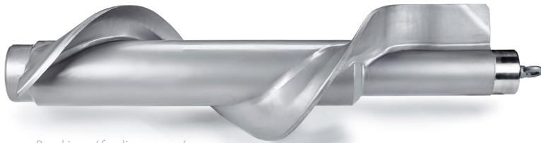
Breaking- / feeding worm/auger
